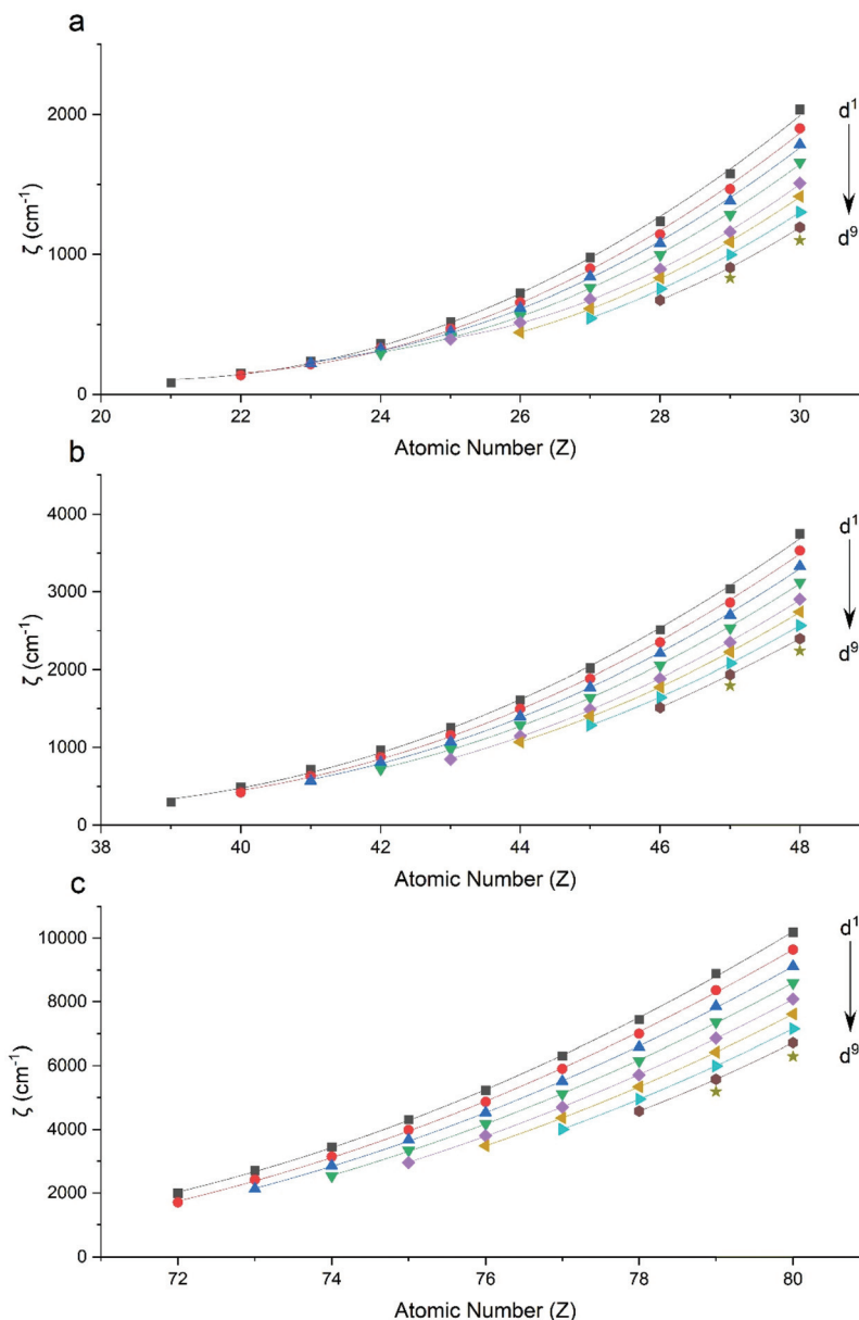
Fig. 1 CASSCF-SO-calculated SO coupling parameters (points) for free ions (a) 3d, (b) 4d, (c) 5d. Lines are second-order polynomial fits, with parameters given in Table S5.†
