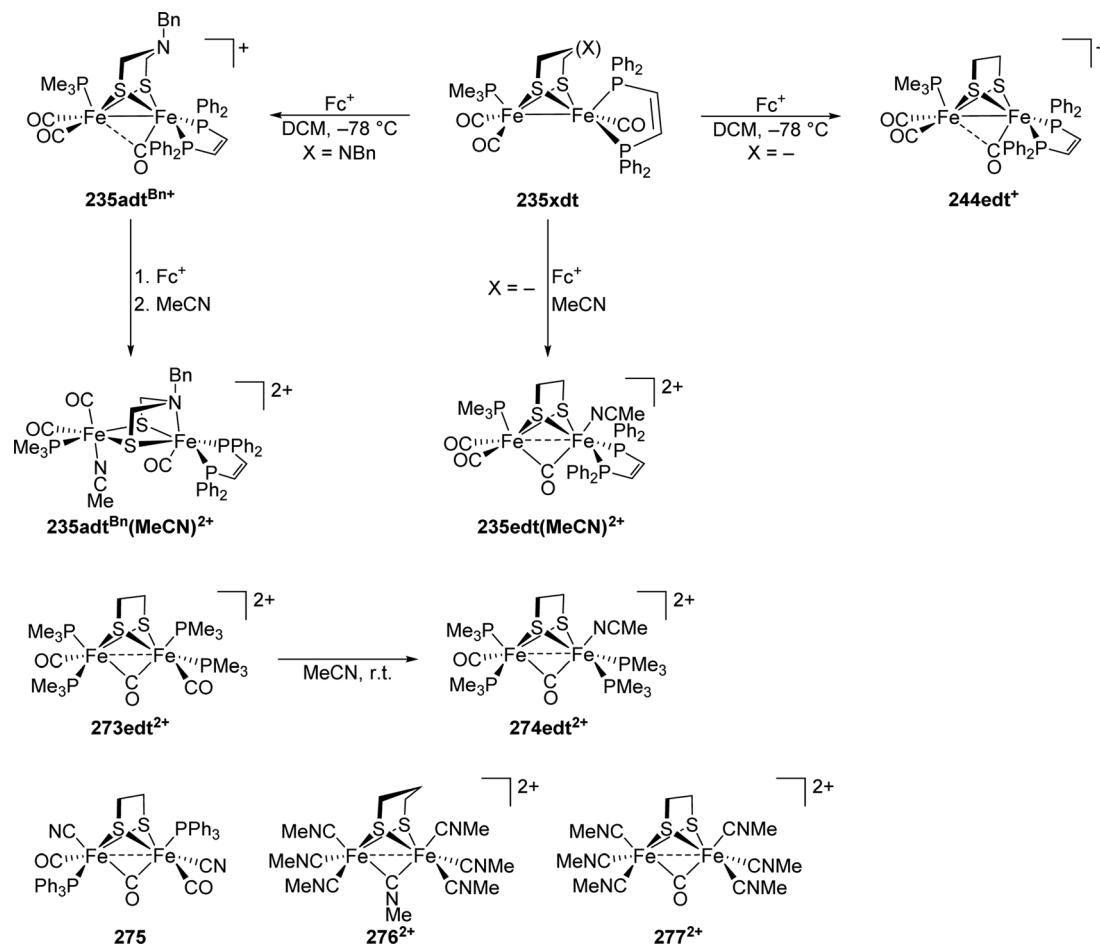
Fig. 83 Top: Oxidation of complex 235adt in the presence and absence of coordinating solvents. Middle: Substitution of a carbonyl ligand in a diferrous complex. Bottom: Exemplary complexes obtained by oxidatively induced ligand substitution.
