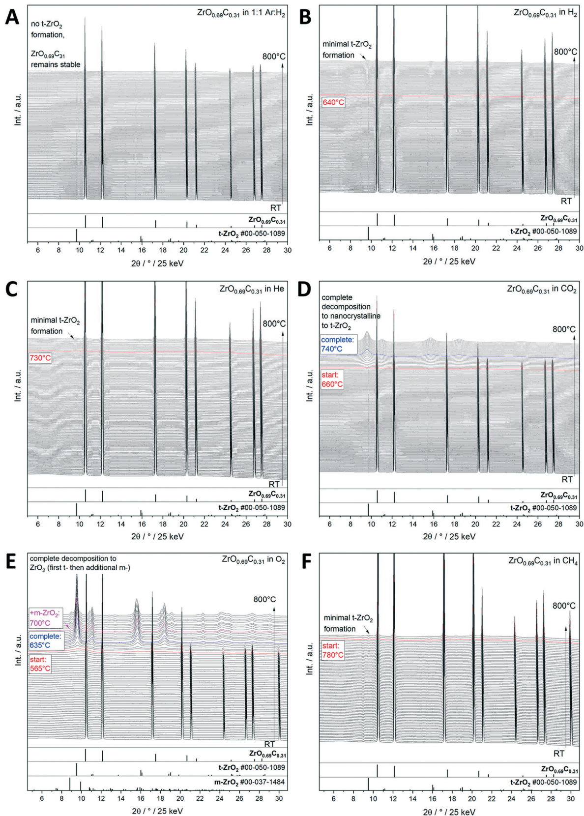
Fig. 3 Decomposition study of crystalline ZrO 0.69 C 0.31 in selected inert, oxidative and reductive gas atmospheres up to 800 °C as monitored by synchrotron-based in situ X-ray diffraction. Panel A: Ar : H 2 mixture = 1 : 1, panel B: pure H 2 , panel C: pure He, panel D: pure CO 2 , panel E: pure O 2 , and panel F: pure CH 4 . The X-ray diffraction patterns are shown as waterfall plots. The temperatures where important structural changes are observed are marked accordingly. Reference patterns are indicated as bars below the diffractograms. In part reproduced with permission from ref. 12 Wiley-VCH, 2021.
