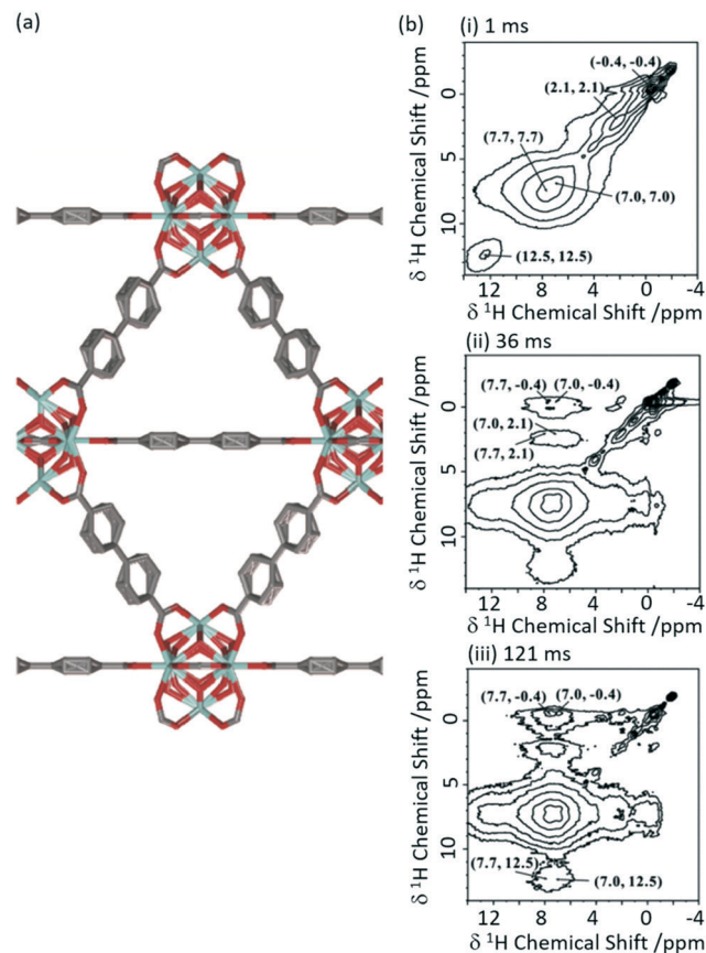
Fig. 7 (a) Schematic structure of \text{UiO-67} . (b) 2D ^1\text{H} - ^1\text{H} spin-diffusion spectra of methane loaded \text{UiO-67} at mixing times of (i) 1 ms, (ii) 36 ms and (iii) 121 ms obtained at a MAS rate \nu_r = 10 kHz. Reprinted (adapted) with permission from ref. 57. Copyright 2017 American Chemical Society.
