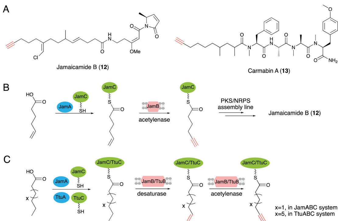
Fig. 6 (A) Structures of 12 and 13 . (B) The biosynthetic pathway for the C 6 alkyne starter unit generation and incorporation into jamaicamide B. (C) Terminal alkyne biosynthetic pathways of JamABC and TtuABC that modify C 6 and C 10 fatty acids, respectively.
