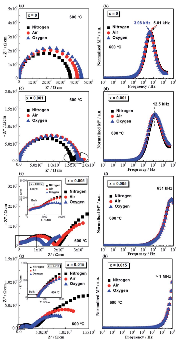
Fig. 3 Impedance spectroscopy data of \text{Na}_{0.5}\text{Bi}_{0.5}\text{Ti}_{1-x}\text{Mg}_x\text{O}_{3.015-x} ( x = 0, 0.001, 0.005 and 0.015 ) ceramics at 600^\circ\text{C} in flowing nitrogen, air and oxygen in the frequency range from 1 MHz to 0.1 Hz. (a), (c), (e) and (g): Z'' plots for x = 0, 0.001, 0.005 and 0.015 , respectively. Inset figures in (e) and (g) are an expanded view of the region in the rectangle. (b), (d), (f) and (h): M'' - \log f spectroscopic plots for x = 0, 0.001, 0.005 and 0.015 , respectively. The numbers inside each figure indicate the frequency at the M'' maxima.
