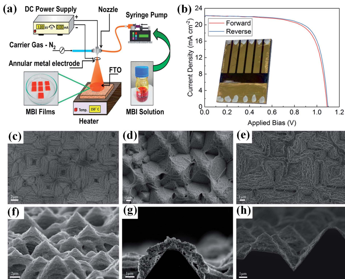
Fig. 26 (a) Schematic illustration of spray coating process with the application of DC voltage used in the fabrication of lead free \text{MA}_3\text{Bi}_2\text{I}_9 perovskite thin films. Reproduced by permission ref. 170, Copyright 2019 International Solar Energy Society. (b) J–V characteristics for the spraycast triple-cation PSC showing 17.8% efficiency in reverse scan. The device photograph is shown in inset. Reproduced by permission ref. 167, Copyright 2018 American Chemical Society. Top-view and cross-section SEM images of the spray-coated films onto the textured silicon bottom cell. (c and f) \text{PbI}_2 NC ink, (d and g) \text{MAPbI}_3 perovskite, and (e and h) \text{CsFAMAPbI}_{3-x}\text{Br}_x mixed perovskite films after spray conversion. Reproduced by permission ref. 169, Copyright 2020 Wiley-VCH Verlag GmbH & Co. KGaA, Weinheim.
