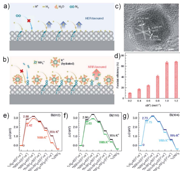
Fig. 6 Mass transfer of \text{H}^+ and \text{N}_2 to the catalyst surface in electrolytes (a) without and (b) with \text{K}^+ . (a) In acidic solutions without \text{K}^+ , \text{H}^+ can be transferred to the surface readily, and the HER will dominate. (b), \text{K}^+ hinders \text{H}^+ transfer to the catalyst surface. \text{N}_2 will be adsorbed preferentially, and the NRR is promoted. (c) High-resolution TEM image of BiNCs, showing the exposed surfaces of {012}, {104} and {110}. (d) FE vs. c(\text{K}^+) . Gibbs free-energy diagrams for the NRR on (e) Bi(012), (f) Bi(110), and (g) Bi(104) facets in the presence or absence of \text{K}^+ (pH 0 and U = 0 V vs. SHE). Reproduced from ref. 124 with permission from the Nature Publishing Group, copyright 2019.
