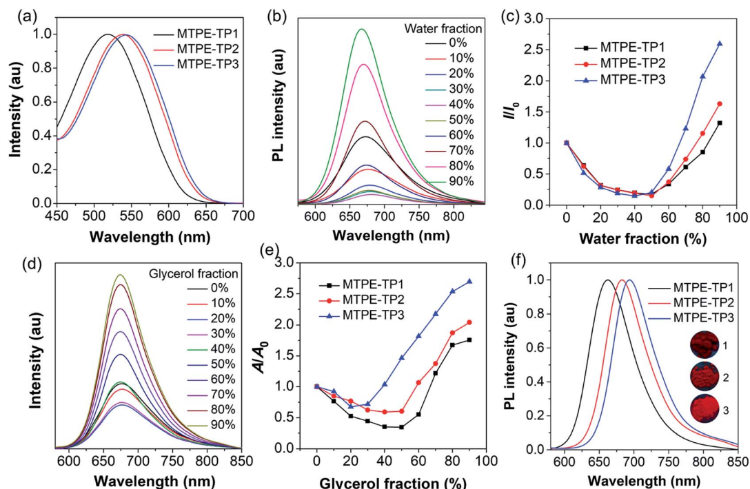
Fig. 2 (a) Absorption spectra of MTPE-TP1-3 in DMSO ( 10^{-5} M). (b) PL spectra of MTPE-TP3 and (c) plot of the PL peak intensity versus water fraction ( f_w ) in DMSO/water mixtures ( 10^{-5} M). I_0 and I represent the PL intensities of the compounds in pure DMSO ( f_w = 0 ) and DMSO/water mixtures with specific f_w s, respectively. (d) PL spectra of MTPE-TP3 and (e) plot of the PL peak intensity versus glycerol fraction ( f_g ) in DMF/glycerol mixtures ( 10^{-5} M). A_0 and A represent the PL intensities of the compounds in pure DMF and DMF/glycerol mixtures with specific f_g s, respectively. (f) PL spectra of MTPE-TP1-3 powders. The inset shows the photographs of powder emission under UV light (365 nm) irradiation.
