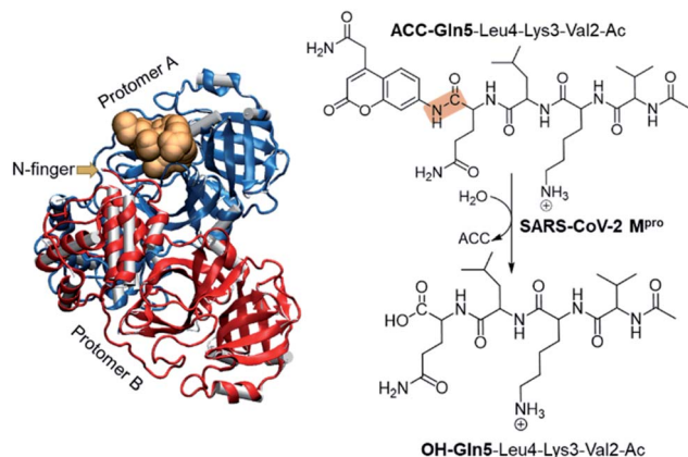
Fig. 1 Structure of dimer SARS-CoV-2 M^{\text{pro}} and the substrate in an active site (gold balls), together with the schematic representation of the SARS-CoV-2 M^{\text{pro}} catalyzed reaction. The scissile peptide bond between Gln5 and ACC is highlighted in orange.
