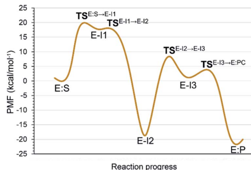
Fig. 2 M06-2X:AM1/MM free energy profile of the proteolysis reaction catalyzed by SARS-CoV-2 M^{\text{pro}} .
