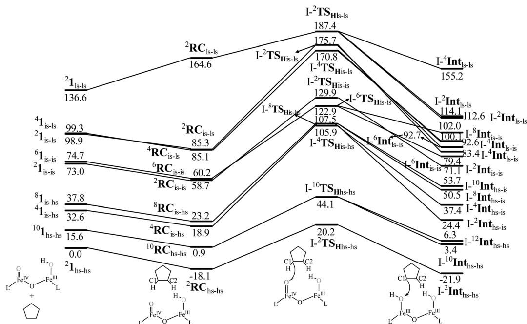
Fig. 2 B3LYP-D3 computed energy profile for the C-H bond hydroxylation of cyclopentane (CP) by species 1 (energies are in \text{kJ mol}^{-1} ).
