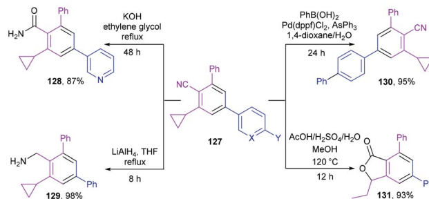
Scheme 36 NHC-catalyzed [4 + 2] benzannulation to synthesize cyano-bearing functional benzenes.
