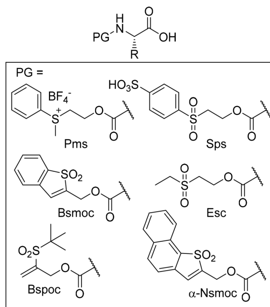
Fig. 5 Water-soluble sulfone-derived amino acid protecting groups developed by Hojo et al. 42,82,84 and Carpino et al. 86,89,90,94
