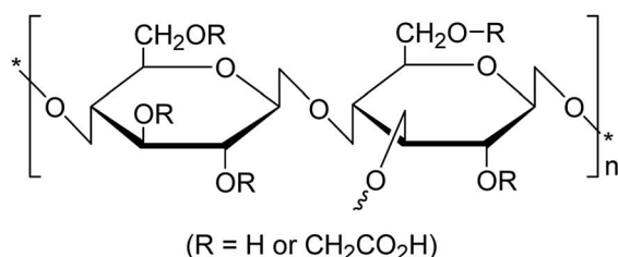
(R = H or CH 2 CO 2 H)
