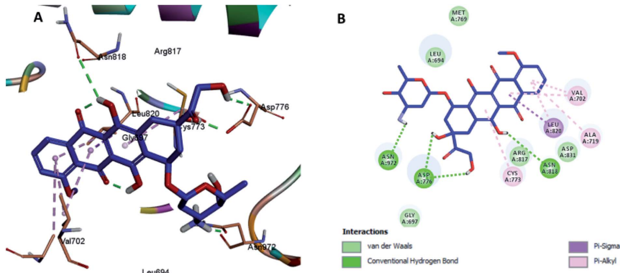
Fig. 3 Docking and binding pattern of DOX in the active site of the HER-2 receptor (PDB entry: 5jeb) (blue). (A) 3D structure of DOX, (B) 2D structure of DOX.
