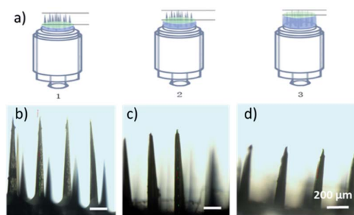
Fig. 2 (a) Length adjustment scheme. (b–d) Microneedle (MN) micrographs when using 50, 100, and 150 \mu L of spacer.
