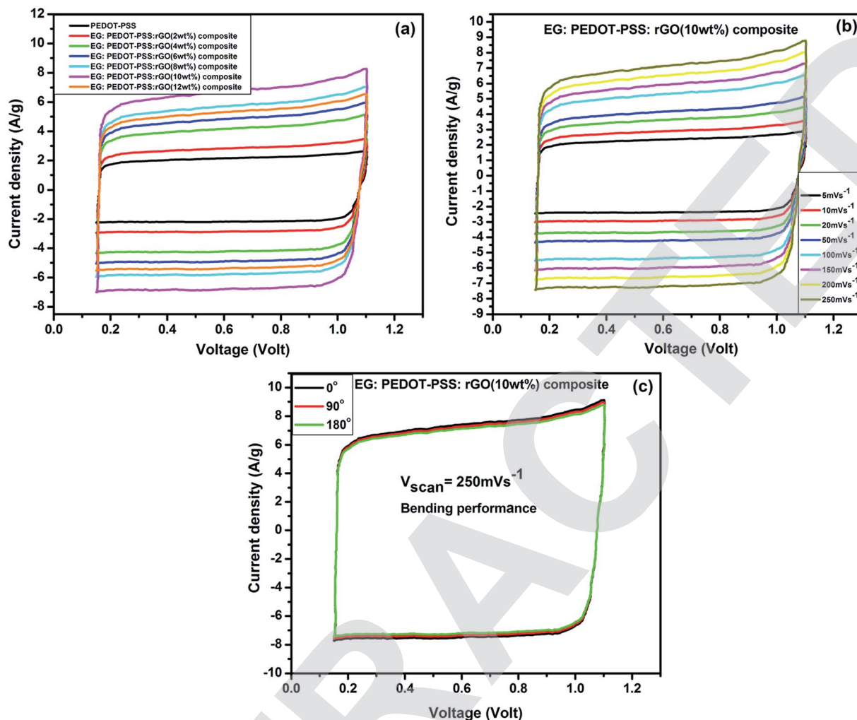
Fig. 7 (a) Cyclic voltamograms for pure PEDOT-PSS and doped PEDOT-PSS thin films (at the scanning rate of 100 \text{ mV s}^{-1} ), (b) CV curves for EG:PEDOT-PSS with 10 wt% of rGO composites at different scanning rates, (in acetonitrile solution containing 1 M \text{LiClO}_4 in the voltage range 0 to 1.2 V), (c) bending C-V performance of EG:PEDOT-PSS with 10 wt% of rGO composites at different angles.
