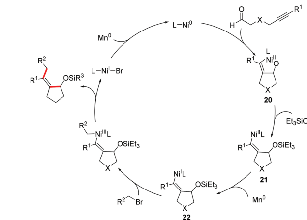
Scheme 17 Ni-Catalyzed reductive coupling of alkynals with alkyl halides.
