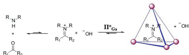
Fig. 24 Synthesis and encapsulation of iminium cation by cage \text{II}^{\text{Ga}} . Reproduced with permission from ref. 13. Copyright 2006, American Chemical Society.
