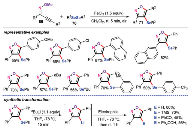
Scheme 31 \text{FeCl}_3 -mediated intramolecular cyclization of alkynone O -methyloximes.
