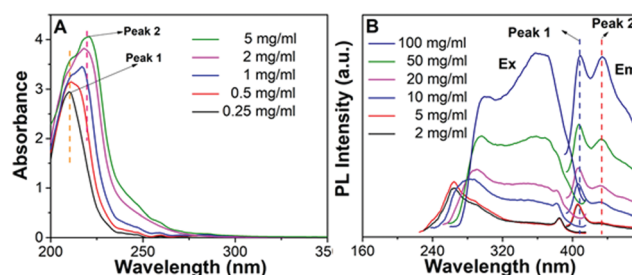
Fig. 2 (A) UV-vis absorption spectra of P1 ethanol solution with the concentration increased from 0.25 \text{ mg mL}^{-1} to 5 \text{ mg mL}^{-1} ; (B) excitation ( \lambda_{\text{em}} = 406 \text{ nm} ) and emission ( \lambda_{\text{ex}} = 360 \text{ nm} ) spectra of P1 ethanol solution with the concentration increased from 2 \text{ mg mL}^{-1} to 100 \text{ mg mL}^{-1} .
