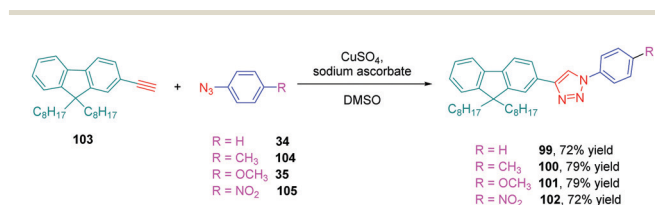
Scheme 11 Click chemistry reaction of four fluorene-triazole-pull molecules 99–102 .
