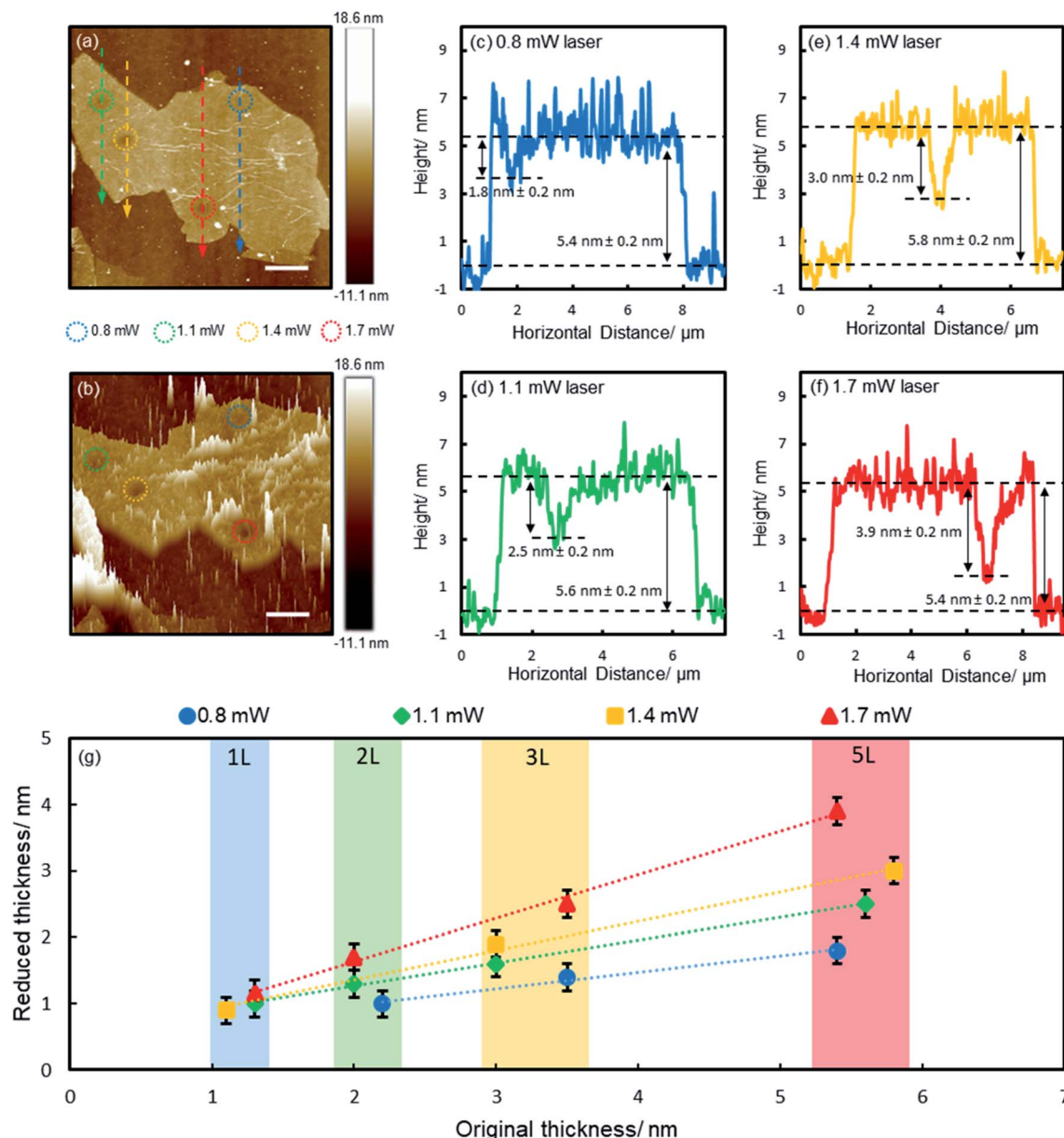
Fig. 2 Reducing GO films with laser irradiation. (a) AFM topographic image of a 5-layer GO film. The irradiated spots are marked by circles. Scale bar: 2 \mu m. (b) 3D plot of (a). (c–f) AFM height profiles along the dashed lines in (a). (g) Reduced film thickness vs. the original GO film thickness. Shaded areas indicate the thickness range of each flake.
