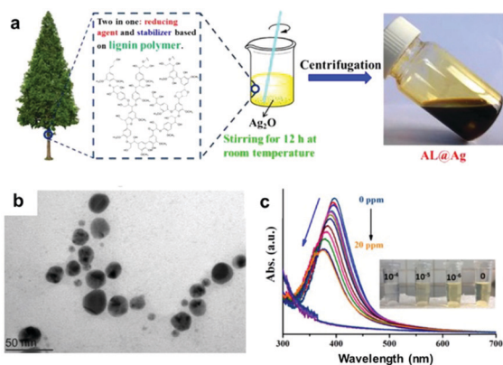
Fig. 6 LNPs as sensor materials: (a) schematic preparation of alkali lignin-coated silver NPs (AL@Ag); (b) a TEM image of AL@Ag particles; (c) UV-vis spectra of AL@Ag particles as sensors for \text{Hg}^{2+} (from 0 to 20 ppm of \text{Hg}^{2+} ) with a decreasing UV-absorption with increasing \text{Hg}^{2+} concentrations, and photographs of the color change process demonstrating the detection \text{Hg}^{2+} at low concentration ( 10^{-4} \text{ M} ). Adapted with permission from ref. 135. Copyright © 2018, American Chemical Society.
