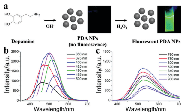
Fig. 1 (a) Schematic illustration of the fluorescent PDA NP synthesis. (b) One-photon emission spectra of fluorescent PDA under different excitation wavelengths. (c) Two-photon emission spectra of fluorescent PDA under different excitation wavelengths. 55 Reproduced from ref. 55 with permission from the Royal Society of Chemistry.
