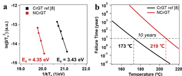
Fig. 7 (a) Kissinger plots for the activation energy calculation of the CrGT and NCrGT films and (b) temperature-dependence of failure time to 10% for the CrGT and NCrGT films.
