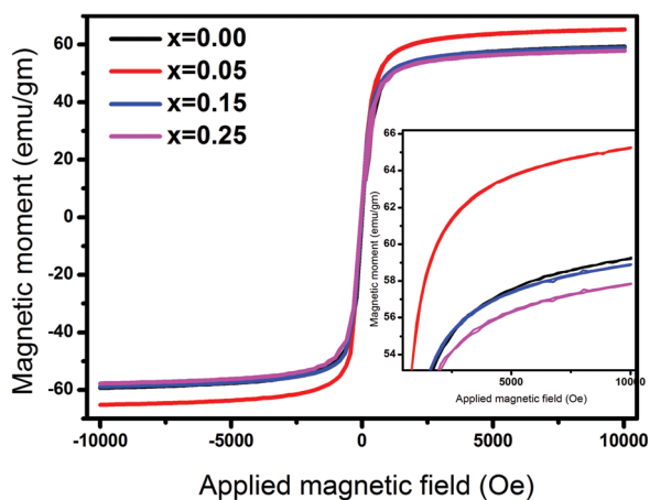
Fig. 7 M - H plots for \text{Ni}_{0.70-x}\text{Cu}_x\text{Zn}_{0.30}\text{Fe}_2\text{O}_4 ( x = 0.00, 0.05, 0.15, \text{ and } 0.25 ) obtained at 300 K.
