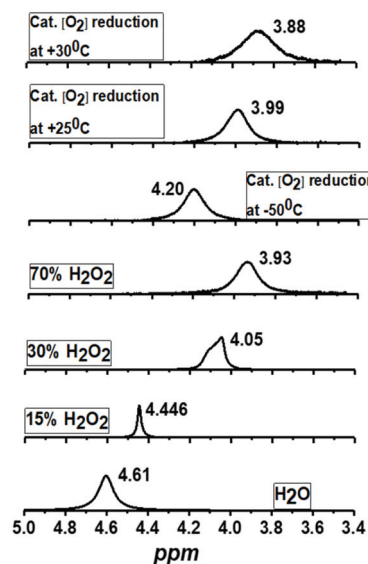
Fig. 5 ^1\text{H-NMR} spectra of the products formed during the complex \text{Co}_4\text{L1} catalyzed dioxygen reduction reactions at 25 °C, 30 °C and –50 °C [ \text{Co}_4\text{L1} (0.01 mM), \text{Fc}^* (3 mM), TFA (10 mM) and \text{O}_2 (0.18 mM)] in acetone- d_6 and comparison with authentic samples containing 70%, 30%, 15% and 0% (weight percent \text{H}_2\text{O}_2 basis) \text{H}_2\text{O}_2/\text{H}_2\text{O} mixtures. All the ^1\text{H} -measurements were performed at 25 °C. The results obtained for \text{Co}_4\text{L1} are then compared with that for \text{Co}_6\text{L2} in Table 2.
