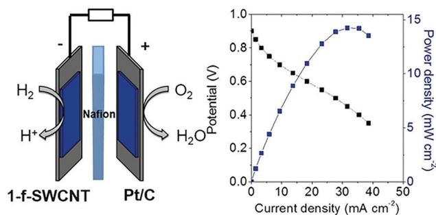
Fig. 11 Polarization (black) and power density (blue) curves for an MEA employing [\text{Ni}(\text{P}^{\text{Arg}}\text{N}^{\text{Arg}})_2]^{7+} (denoted as 1-f-SWCNT) and Pt/C as the anode and cathode catalysts, respectively. Experimental conditions: anode loading: 0.3\text{ }\mu\text{g cm}^{-2} , cathode loading (Pt/C): 1\text{ mg cm}^{-2} , Nafion ® as the polymer electrolyte, 60\text{ }^\circ\text{C} cell temperature. Reprinted with permission from ref. 297. Copyright 2017 Wiley-VCH.
