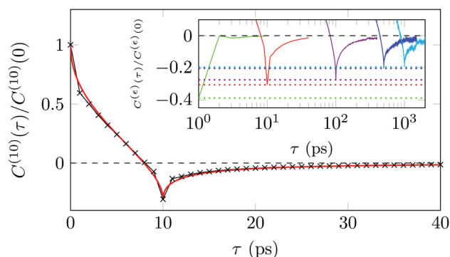
Fig. 14 Measured displacement-autocorrelation function (black crosses) compared with the theoretical FBM prediction for \alpha = 0.47 and \epsilon = 10 ps (red line). The inset shows the dependence of the measured displacement autocorrelation function on the binning size \epsilon for values of \epsilon of 1 ps (green), 10 ps (red), 100 ps (violet), 500 ps (blue) and 1000 ps (light blue).
