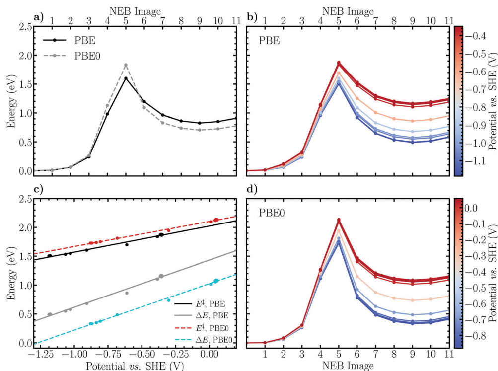
Fig. 4 Comparison of PBE and PBE0 results for the CI-NEB minimum energy profiles of the Heyrovský reaction on the investigated (14,0) NCNT. (a) Optimized PBE energy profile and the re converged profile employing the truncated PBE0 exchange-correlation functional. (b) Charge-extrapolated constant electrode potential energy profiles at the PBE level of theory. (c) Electrode potential dependence of the activation barriers and reaction energies of the Heyrovský reaction based on the charge-extrapolation scheme and the PBE and PBE0 functionals. (d) Charge-extrapolated constant electrode potential energy profiles based on the reoptimized PBE0 results.
