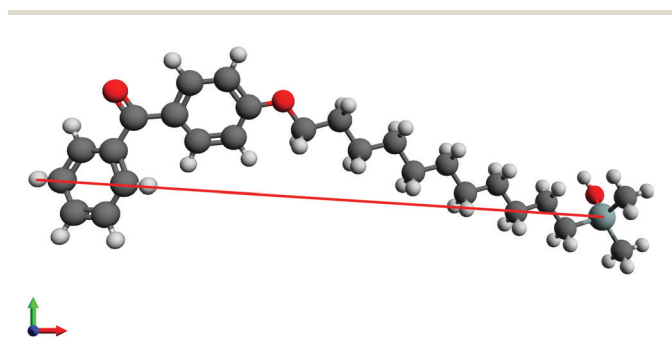
Fig. 1 The ball-and-stick model of 11-BPS in all- trans conformation in an optimized geometry (Avogadro, UFF force field) is shown exemplarily. The red colored line indicates the molecular length measured (23.75 Å). Here, showing the crystal structure of the SiO 2 surface (to which the BPS molecule is attached in a real sample) would reduce the clarity, and hence a covalently bound BPS-O-SiH 3 is shown instead.
