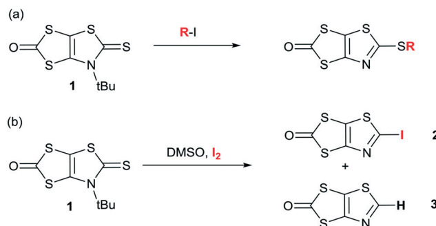
Scheme 2 Synthetic path to the prolignands 2 and 3 .
