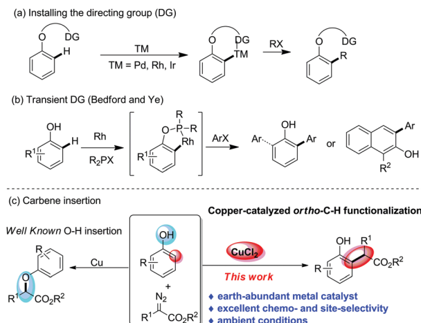
Scheme 1 Ortho -selective C–H functionalization of phenols.
