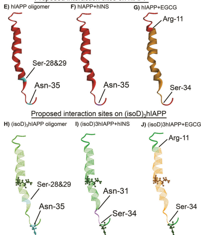
Fig. 2 Summarised fragments of hINS attached to (A) hIAPP and (B) (isoD) 3 hIAPP. Summarised fragments of EGCG attached to (C) hIAPP and (D) (isoD) 3 hIAPP. The proposed interaction sites on (E) pure hIAPP (PDB 2K8B) 21 with (F) hINS and (G) EGCG. The proposed interaction sites on (H) pure (isoD) 3 hIAPP with (I) hINS and (J) EGCG.
