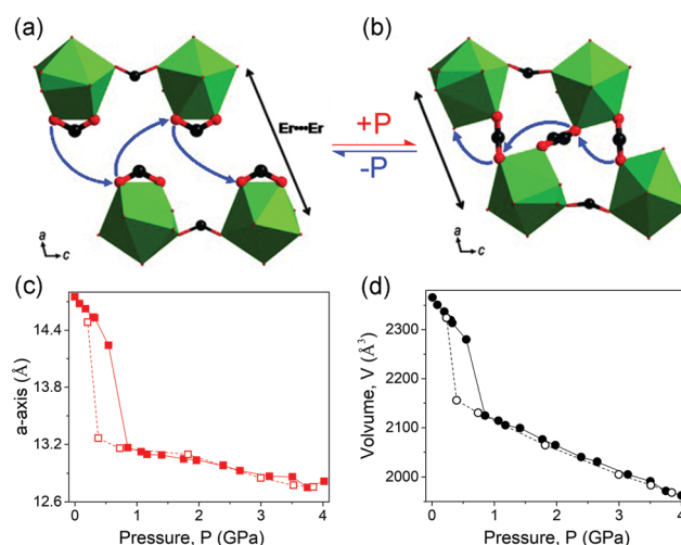
Fig. 19 Partial crystal structure changes of the [\text{tmenH}_2][\text{Er}(\text{HCOO})_4]_2 before (a) and after (b) compression. Lattice parameter changes of a (c) and volume ( d ). The data collected with increasing and decreasing pressure are plotted with filled and empty spheres, respectively. Reprinted with permission from ref. 124.
