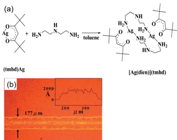
Fig. 16 (a) The synthetic reaction of the [Ag(dien)](tmhd) complex. (b) The optical microscopy image of printed conductive silver lines on flexible PI substrates. Reproduced with permission from ref. 48. Copyright 2013, Royal Society of Chemistry.
