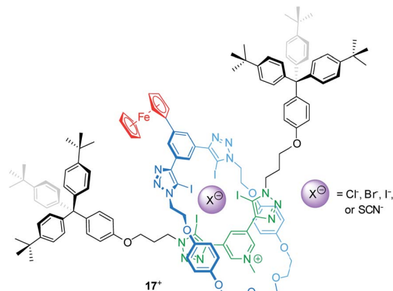
Fig. 14 Structure of the bromide-sensing [2]rotaxane 17^+ , which provides a halogen bonding anion binding cavity.
