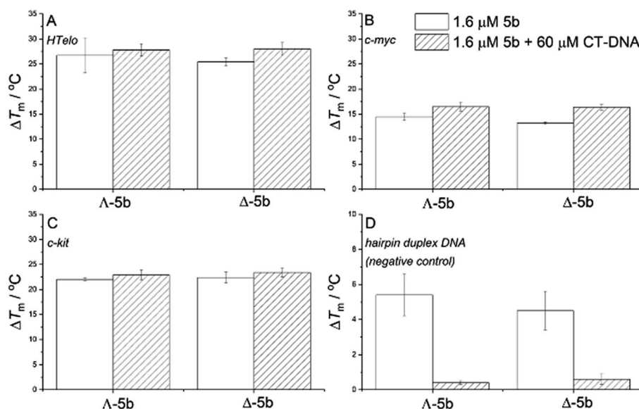
Fig. 8 Selective stabilization of DNA G-quadruplexes over duplex DNA. FRET melting assay of fluorophore-labelled quadruplex-forming oligonucleotides (A) HTelo, (B) c-myc, (C) c-kit, and (D) the labelled oligonucleotide F26T ds -hairpin, which does not form a quadruplex structure (negative control). \Delta T_m values determined by FRET upon addition of 5b (1.6 \mu\text{M} ) in the absence and in the presence of 60 \mu\text{M} CT-DNA show strong preferential quadruplex binding in the presence of excess duplex CT-DNA ( \Delta T_m unchanged).
