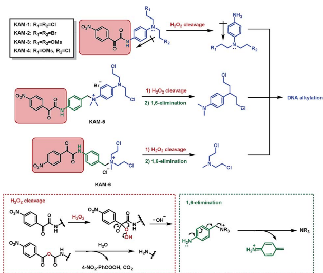
Scheme 1 Structures of KAM prodrugs and the mechanisms of H_2O_2 -responsive activation to generate DNA alkylating agents.
