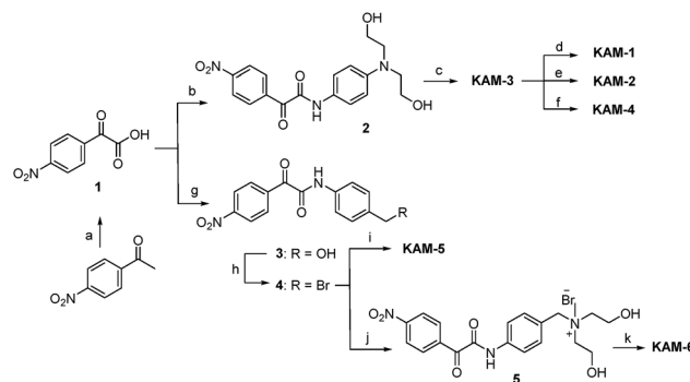
Scheme 2 Synthesis of KAM prodrugs. Reactants and conditions: (a) SeO_2 , pyridine, 90 °C, N_2 , 35%; (b) N -4-aminophenyl diethanolamine, EDCI, DIEA, DMF, 42%; (c) MsCl , DMAP, TEA, DCM, reflux, 70%; (d) LiCl (5 eq.), DMF, 60 °C, 65%; (e) NaBr (5 eq.), DMF, 60 °C, 67%; (f) LiCl (1 eq.), MeCN, 60 °C, 23%; (g) (4-aminophenyl)methanol, EDCI, DIEA, DMF, 33%; (h) CBr_4 , PPh_3 , DCM, 0 °C–r.t., 50%; (i) N -(4- N,N' -dimethylaminophenyl)-bis(2-chloroethyl)amine, MeCN, 43%; (j) N -methyl-diethanolamine, CHCl_3 , reflux, 76%; (k) SOCl_2 , r.t., 62%.
