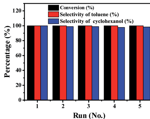
Fig. 9 Catalytic cycling tests of Ni/Al _2 O _3 -600 catalyst during the hydrogenation of benzyl phenyl ether. Reaction conditions: benzyl phenyl ether ( \alpha -O-4) (185 mg, 1 mmol), Ni/Al _2 O _3 -600 (20 mg), solvent (10 mL), 150 °C, stirring at 1000 rpm, 5 h.
