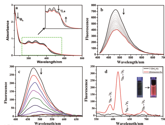
Fig. 2 (a) Absorption spectra and (b) emission spectra of 1 (0.2 mM) with (red) and without (black) \gamma\text{-CD} (0–0.3 mM) at pH 9.0 in water (25 ^\circ\text{C} ). (c) Emission spectra of \gamma\text{-CD} \cdot 1_2 (0.2 mM) upon addition of \text{Eu}^{3+} (from 0 to 3 eq.) at pH 9.0 in water (25 ^\circ\text{C} , \lambda_{\text{ex}} = 365 nm) (d) emission spectra of the \text{Eu}^{3+} \subset \gamma\text{-CD} \cdot 1_2 system (black) and \text{Eu}^{3+} \subset [2]\text{rotaxanes} (red) at 25 ^\circ\text{C} . Inset: photo image of fluorescence in pH 9.0 aqueous solution under UV light ( \lambda_{\text{ex}} = 254 nm, 254 nm used as an excitation source).
