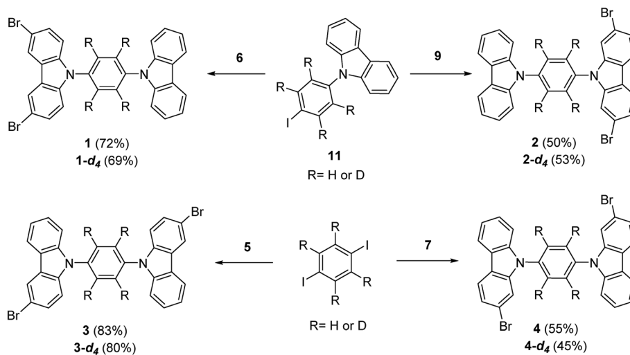
Scheme 1 Synthesis of rotors 1–4 and deuterated analogues, see the ESI† for the synthesis of the precursors.
