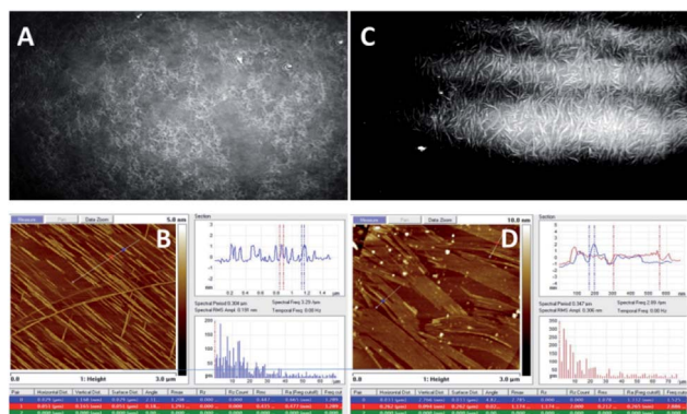
Fig. 5 BAM (sizes 720 × 400 micrometres) and AFM images of the compound 1d . (A) (BAM) and (B) (AFM): before the collapse, at \pi = 13 mN m -1 ; (C) (BAM) and (D) (AFM): after the collapse, at \pi = 27 mN m -1 (see ESI, Fig. ESI-5† for the enlarged AFM images of B and D).
