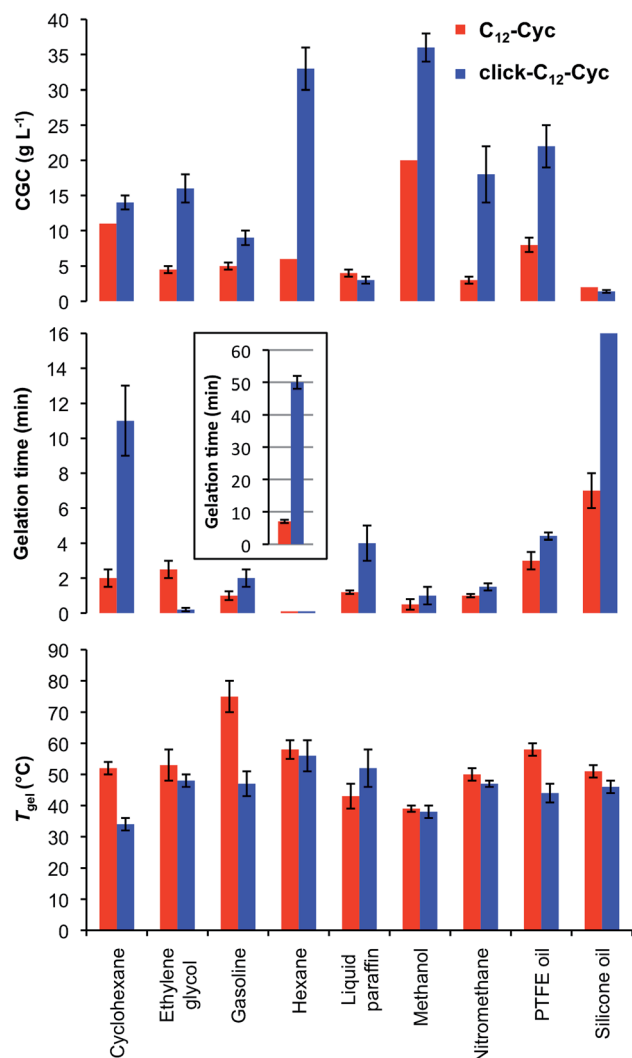
Fig. 4 Comparative plots of the T_{\text{gel}} , gelation kinetics and CGC values for the organogels made of C_{12} -Cyc and \text{click-}C_{12} -Cyc in nine organic solvents. Both the T_{\text{gel}} and gelation time values were estimated at the corresponding CGC values. Inset (middle plot): gelation time in hexane. Each experiment was repeated at least three separate times and the error bars show the SDM.
