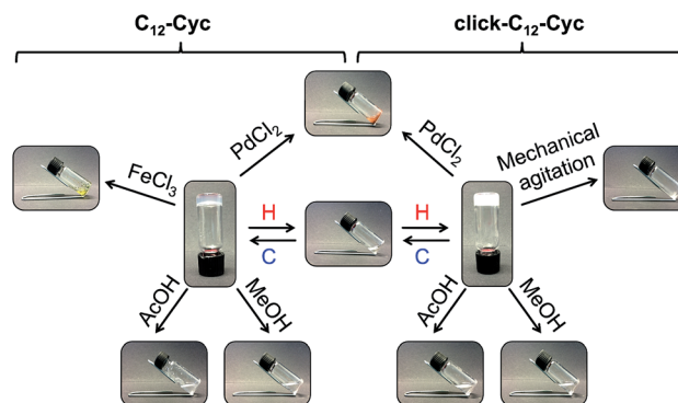
Fig. 5 Representative stimuli responsive map of organogels made of C_{12} -Cyc and \text{click-}C_{12} -Cyc in cyclohexane ( c = 15 \text{ g L}^{-1} ). Abbreviation: H = heating; C = cooling. [\text{AcOH}] = 1 \text{ M} .
