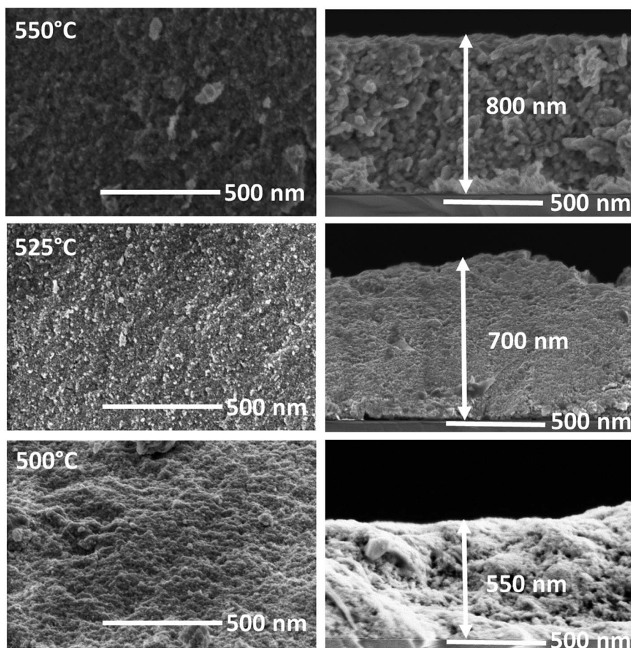
Fig. 5 Planar and cross-sectional FE-SEM images of CZTSSe films at different selenization temperature.
