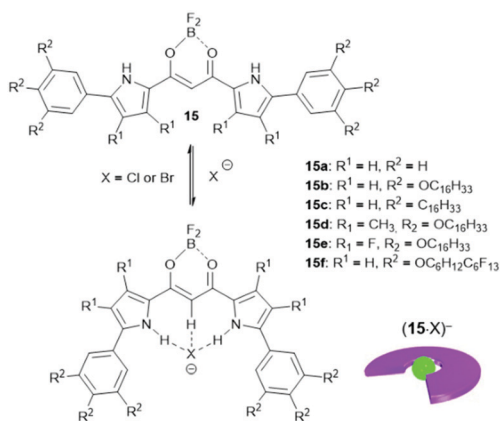
Fig. 12 Schematic representation of the formation of \pi -electronic anions by binding of a halide to the anion receptor 15 .
