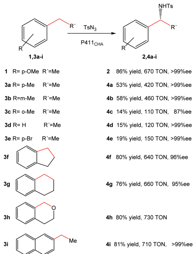
Fig. 4 Substrate range of intramolecular C–H amination catalyzed by cells expressing P411 CHA . The figure is adapted from ref. 22.
