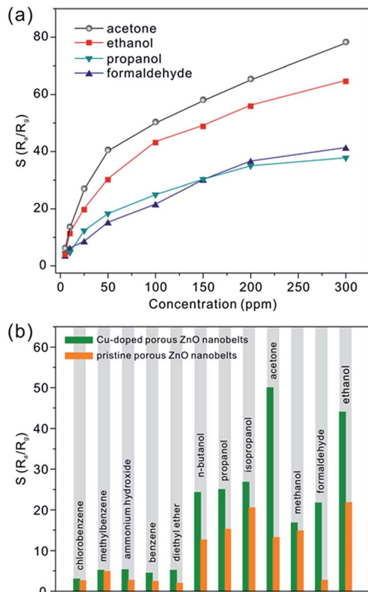
Fig. 7 (a) The relationship between the relative response and the concentration of some typical VOCs (acetone, ethanol, propanol, and formaldehyde), and (b) the relative responses of CZ-3 porous nanobelts toward all investigated VOCs (100 ppm) in contrast to those of pristine porous ZnO nanobelts at the optimal working temperature of 325 °C.
