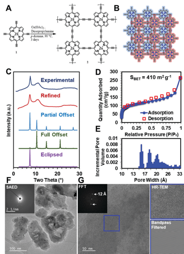
Fig. 4 (A) Synthesis of zinc porphyrin 2D COF; (B) modelled porphyrin COF structure; (C) experimental and simulated PXRD patterns; (D) \text{N}_2 adsorption (closed circles) and desorption (open squares) isotherms (77 K) for 2 , and (E) pore size distribution of 2 . (F) Low-resolution TEM image (inset: SAED pattern of particles) (G) high-resolution TEM image (inset: FFT of boxed region in (G)). Side panels: lattice image of boxed region in (G) and bandpass filtered image of that region of zinc porphyrin 2D COF particles.
